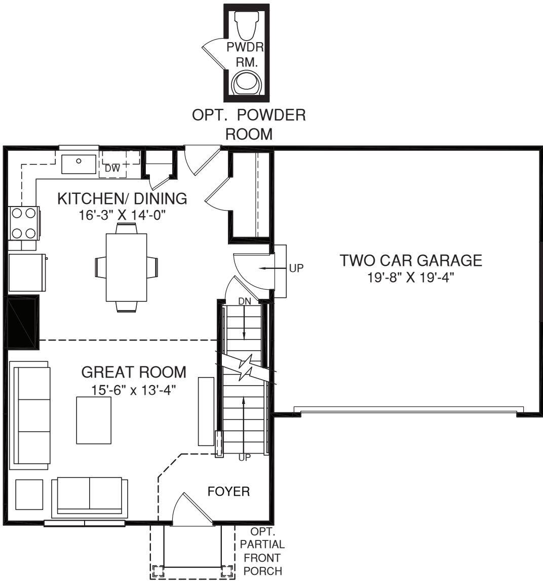
MAIN LEVEL
