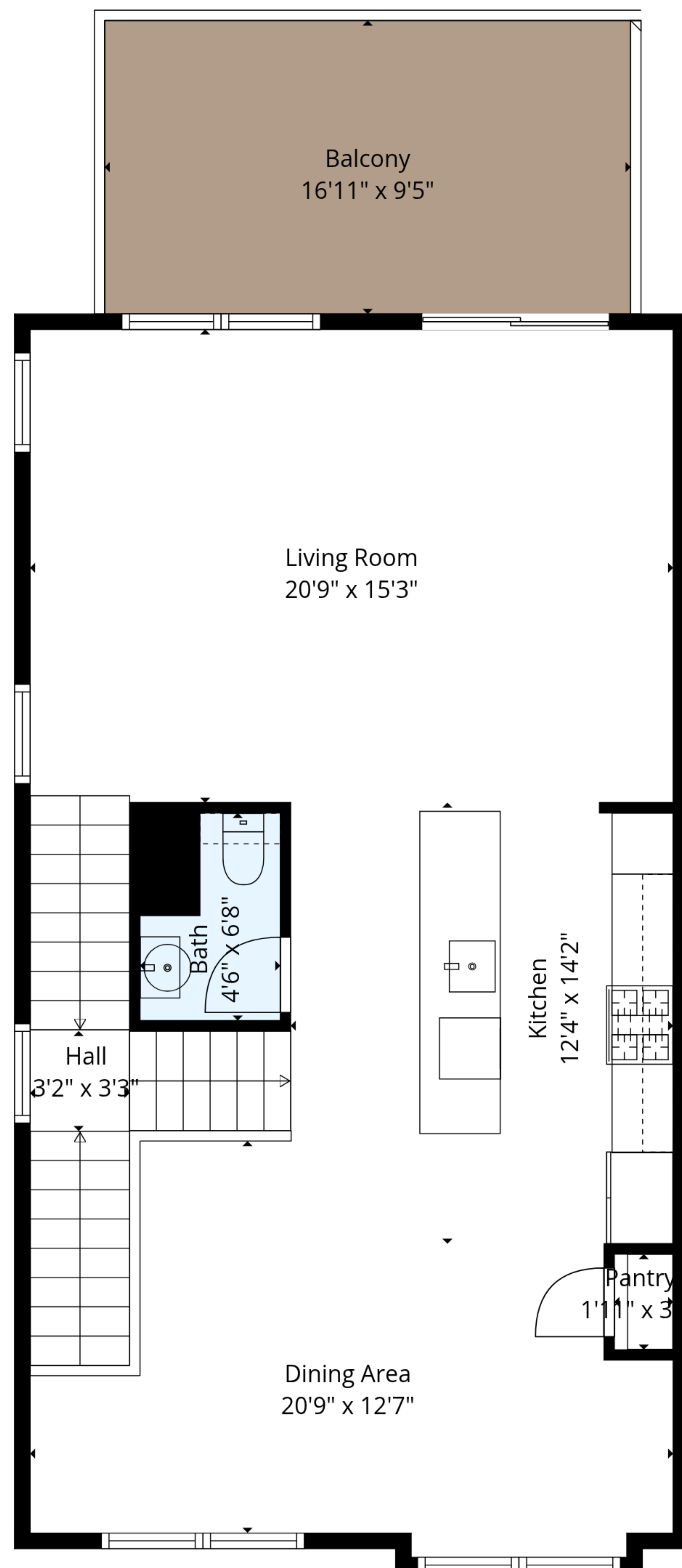
2nd Floor
