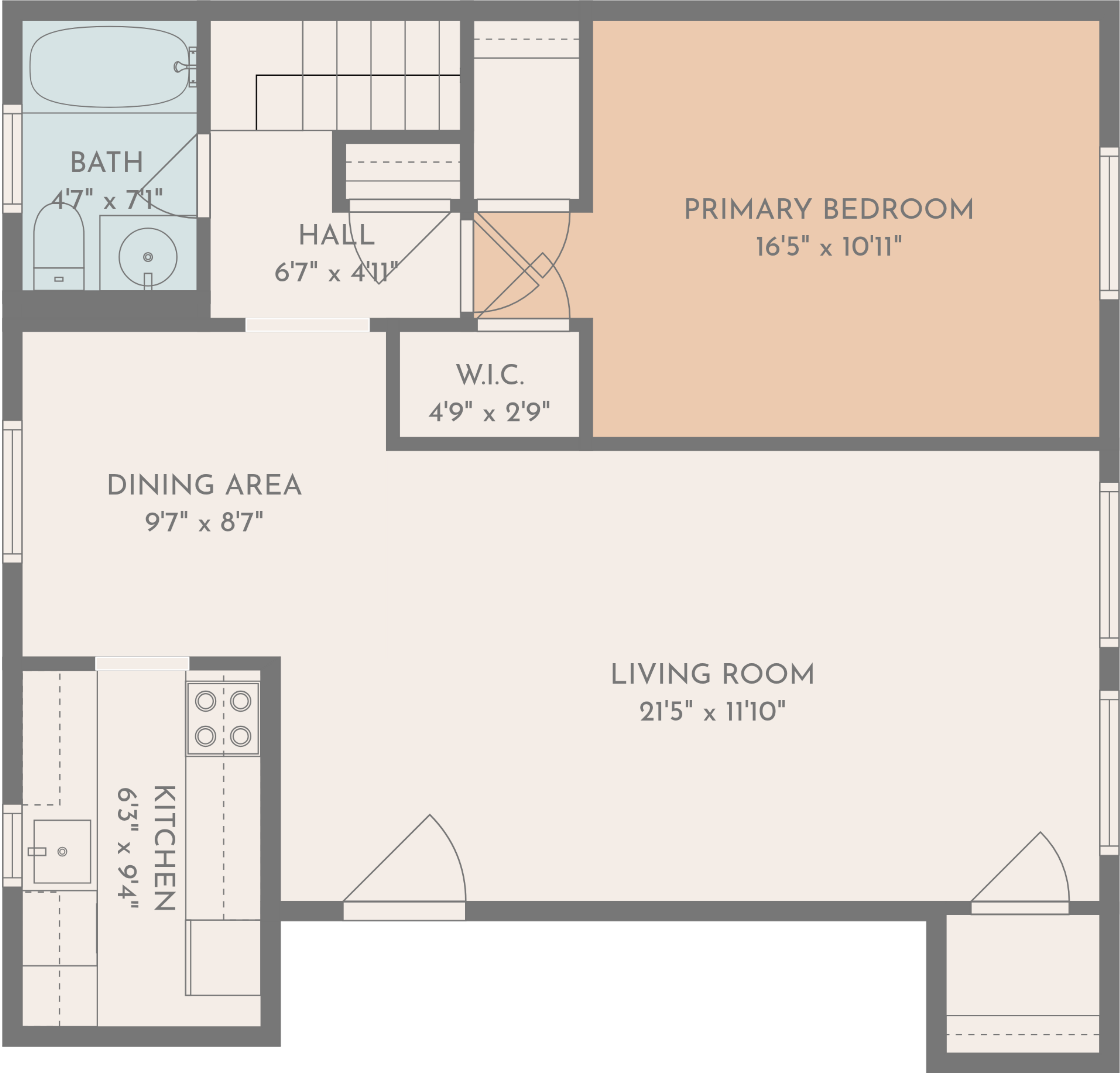
1st floor
