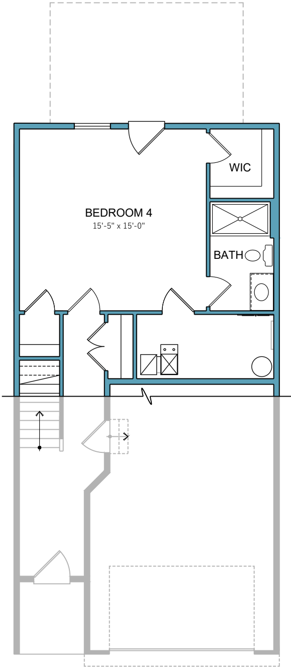
PLAN OPTION 1: GROUND FLOOR PLAN W/ OPTIONAL BEDROOM 4 WITH BATH AND WIC
