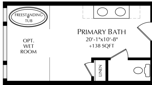
EXT. PRIMARY BATH w/WET ROOM +138 SF TAKES PLACE OF THE SITTING ROOM & EXISTING W.I.C. THE W.I.C. RELOCATES TO THE EXISTING BATH LOCATION
