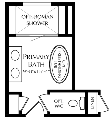
ALT. PRIMARY BATH LAYOUT OPT. ROMAN SHOWER, FREESTANDING TUB & WATER CLOSET
