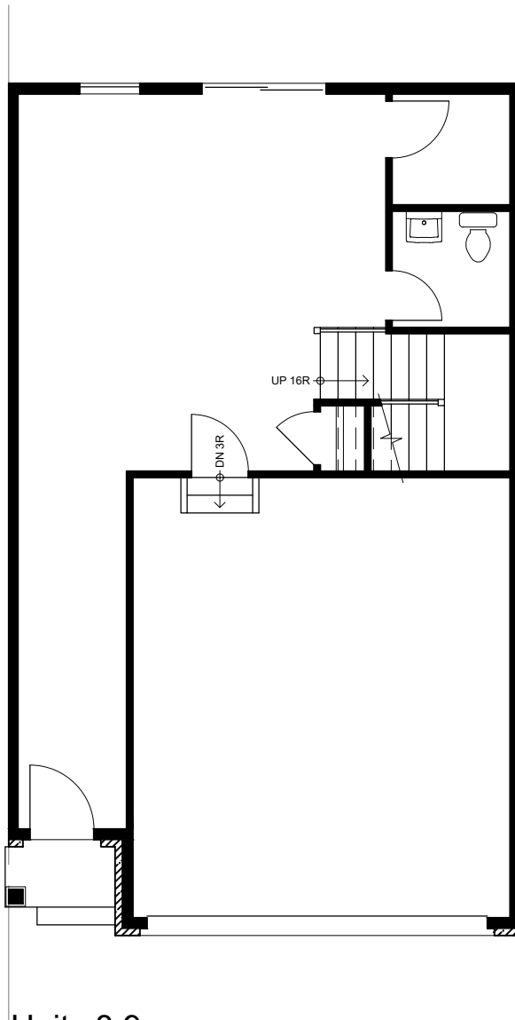
Units 8,9 TYPICAL UNIT TOWNHOUSE FIRST FLOOR PLAN
