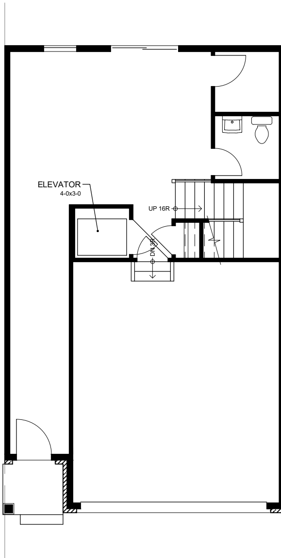
With Elevator TYPICAL UNIT TOWNHOUSE FIRST FLOOR PLAN
