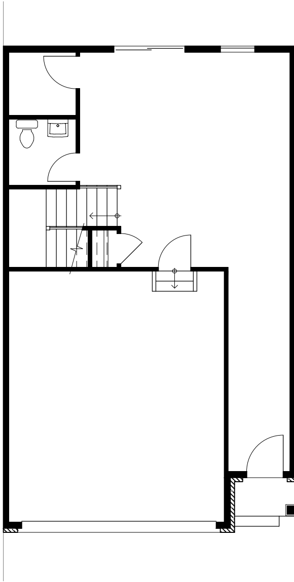
Units 7,9,11 TYPICAL UNIT TOWNHOUSE FIRST FLOOR PLAN
