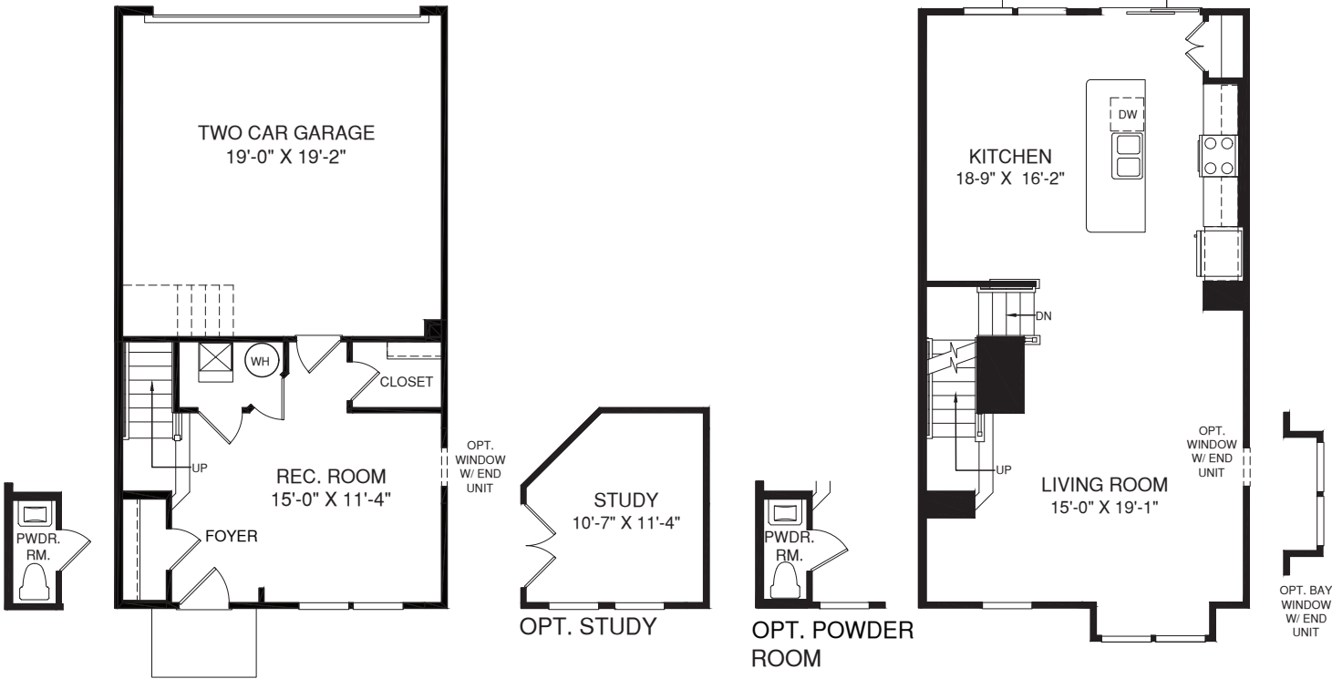
LOWER LEVEL
