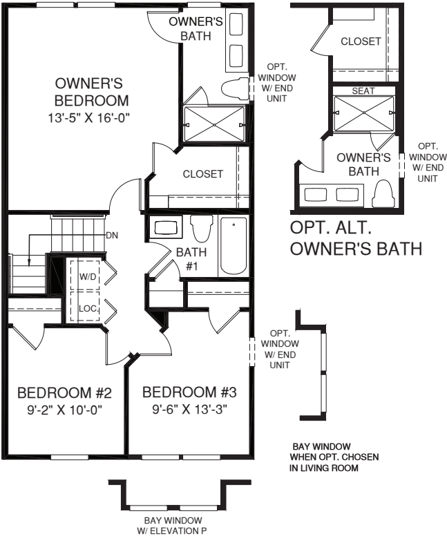
UPPER LEVEL
